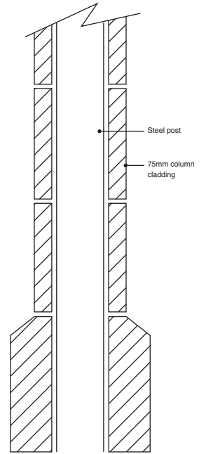
Section
