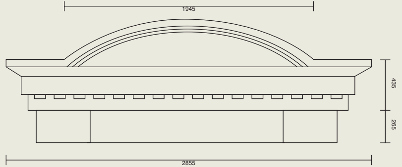
Elevation of front portico
