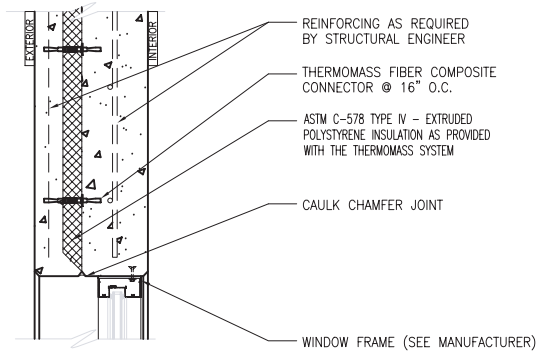
HEAD DETAIL - JAMB SIMILAR
