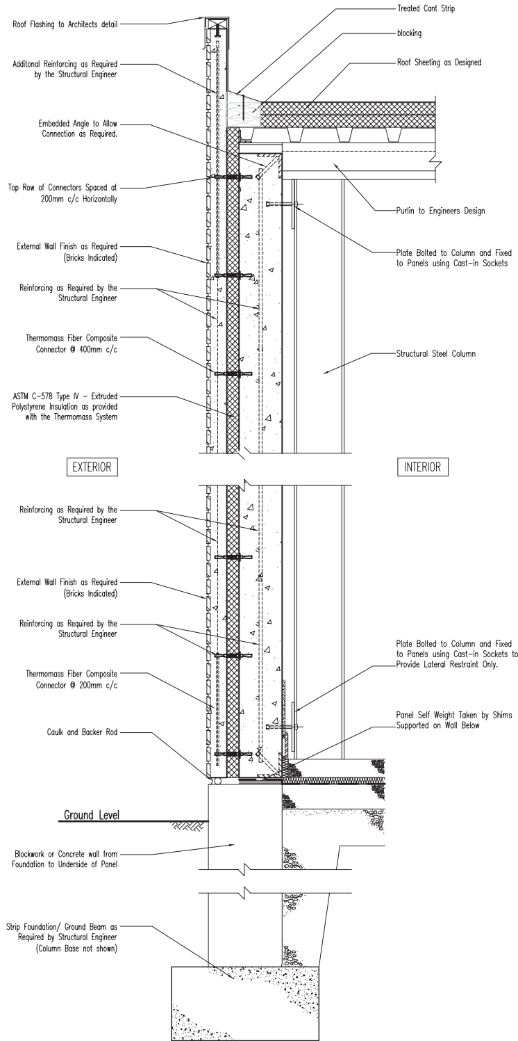
Vertical Section Taken Through Wall at Column Position
