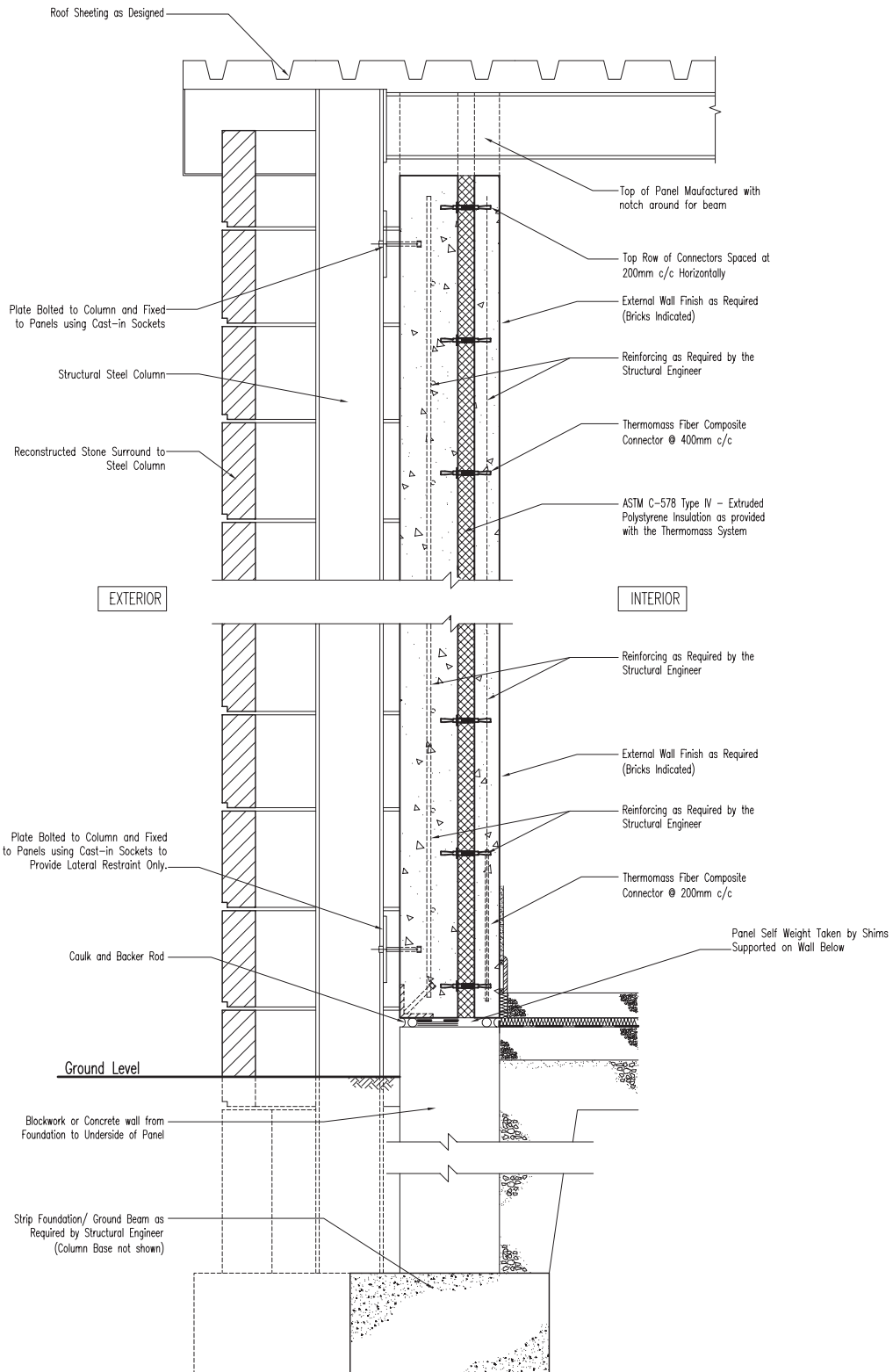
Vertical Section Taken Through Wall with External Column
